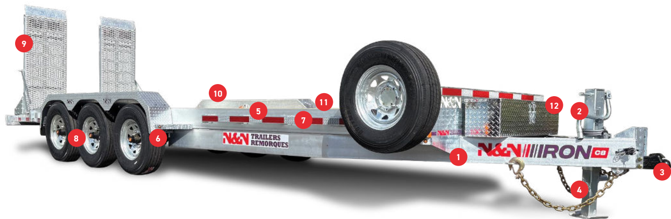
IROC8-724G307 shown with spare tire holder (Add-on)
